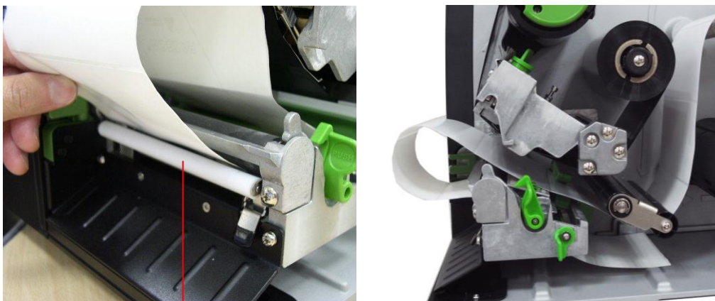
Peel-off roller
